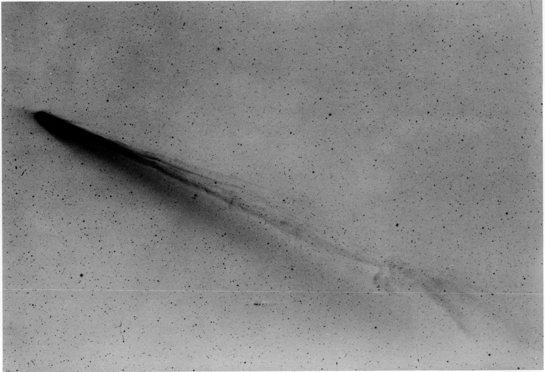
Figure 4. JOCR photograph of comet Kohoutek on January 11, 1974.
